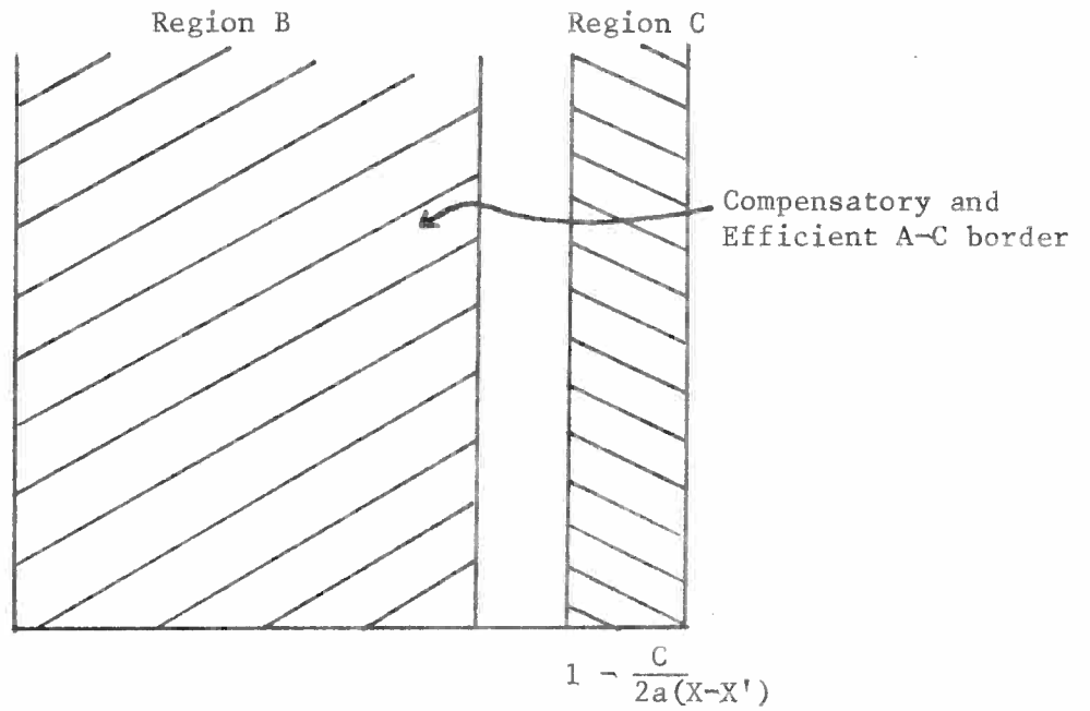
Figure 6 Regions B and C for Liquidated Damages and Linear Technology
