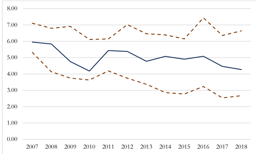
Figure 1 Climate Policy Score Median and inter-quartile range 2007 - 2018
