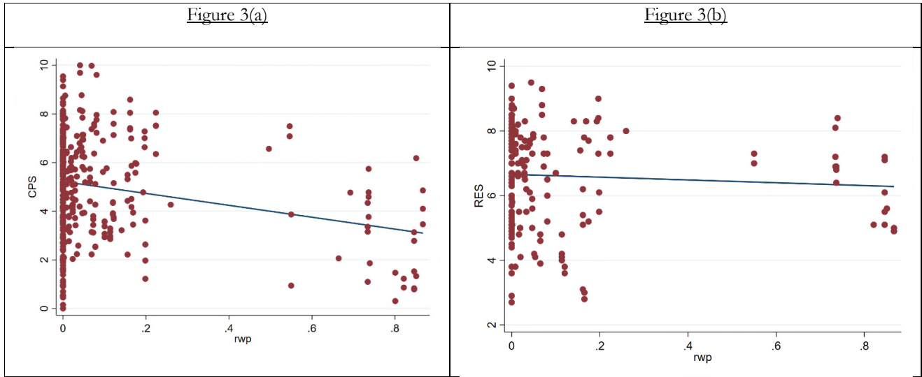
Figure 3 Correlations between rwp and CPS, RES
