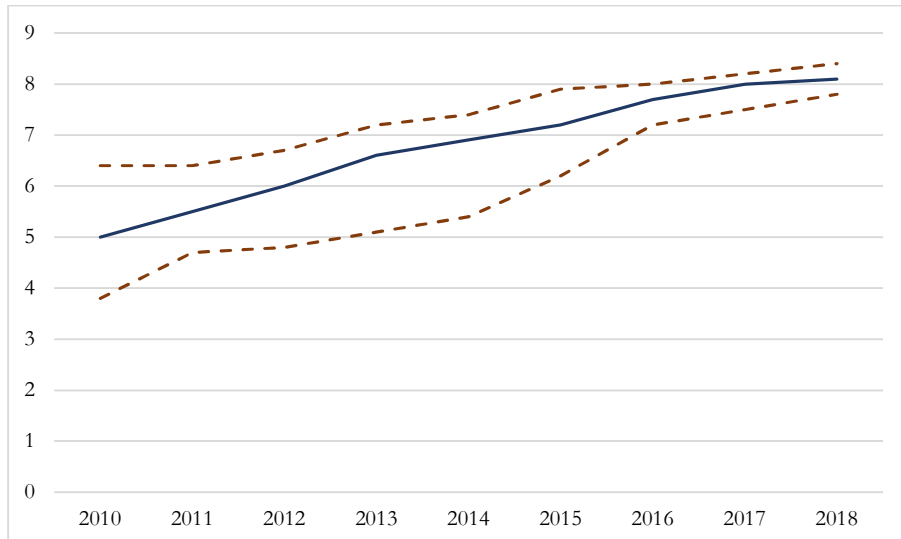
Figure 2 Renewable Energy Score Median and inter-quartile range 2010 - 2018
