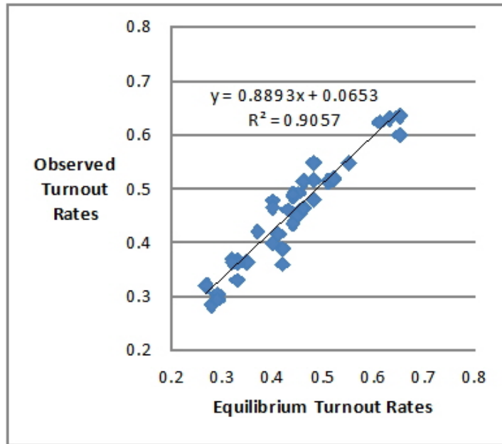
Figure 4: Observed Turnout Rates plotted against QRE-estimated Turnout Rates.
