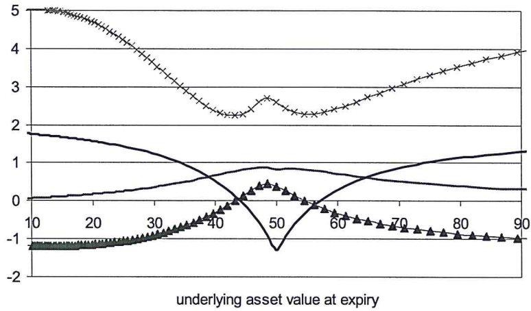
FIGURE 5 Conditional Moments of Hedging Errors in a Binomial Tree with 200 timesteps
