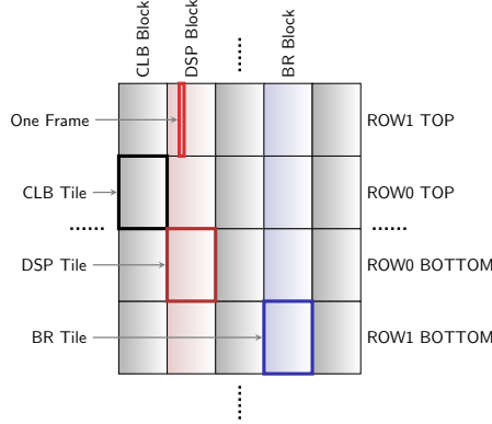
Fig. 1. Virtex 5 FPGA architecture.
